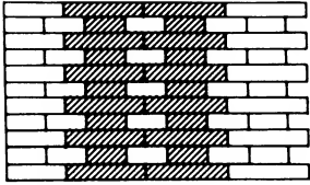
1 English bond
